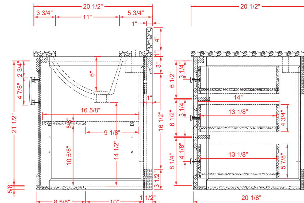
SIDE VIEW
