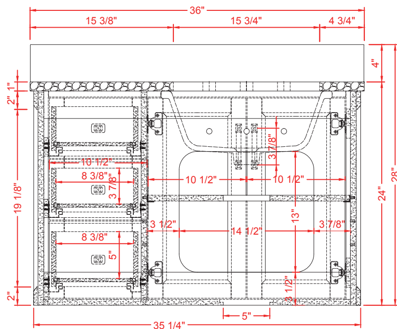
BACK VIEW
