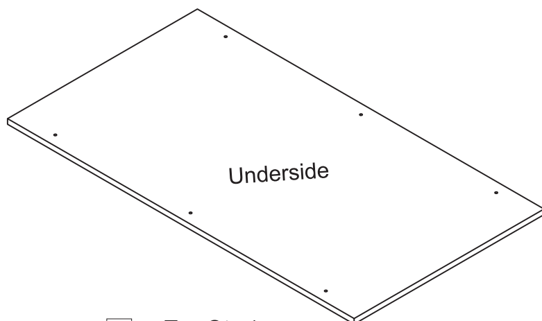
1 Top Qty 1 (42.15x22.99x0.59")
