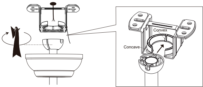
Safety rope installation method
