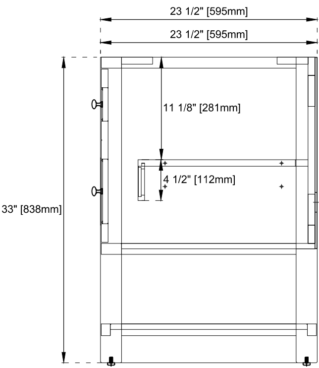
Side View
