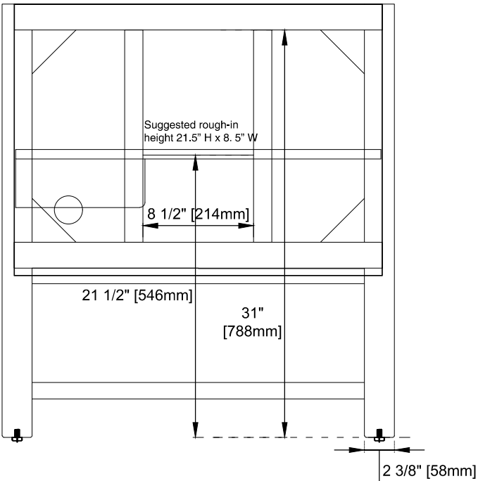
Back View
