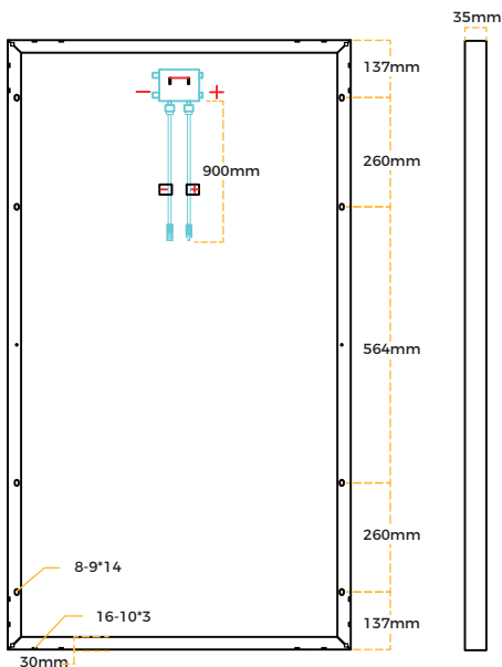
Back Profile (unit mm)
