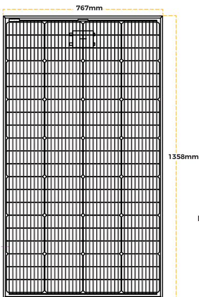
Front Profile (unit mm)
