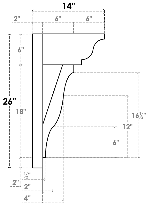
SIDE PROFILE
