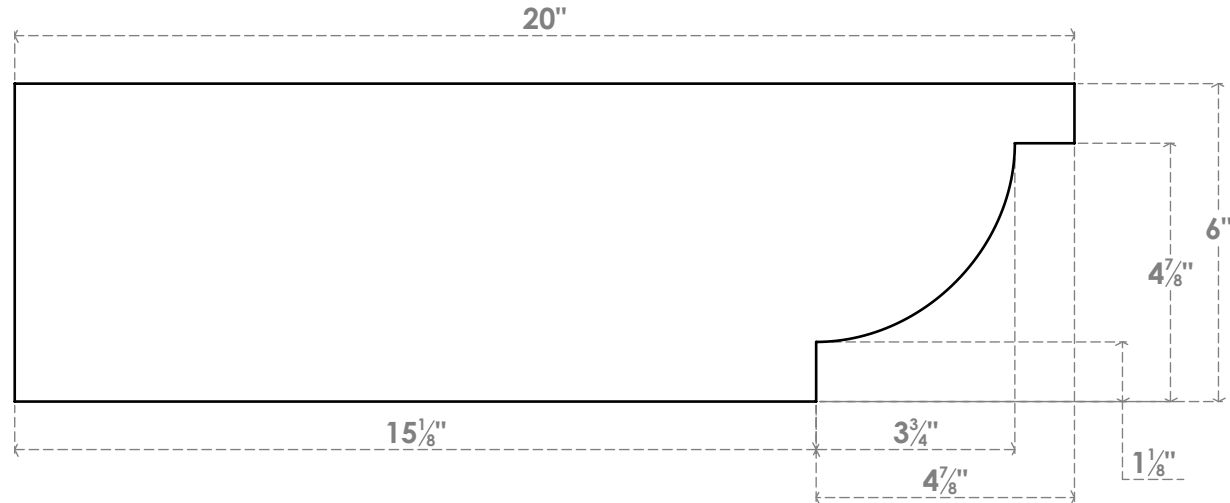
SIDE PROFILE
