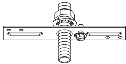
Mounting Strap Unit (A)
