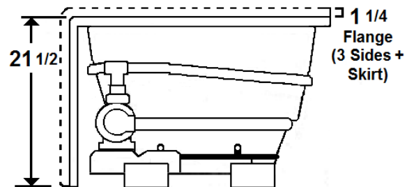
Standard (S) Pump Location
