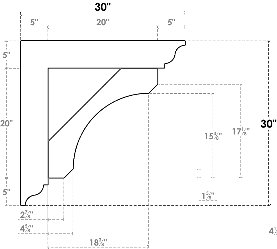
SIDE PROFILE
