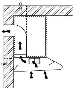
Ducted Mode
