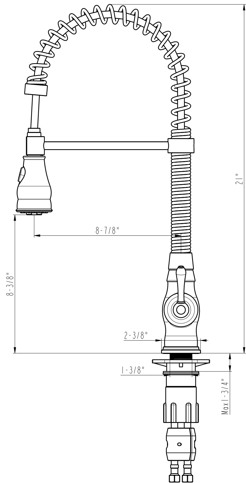
96518A Dimensional Drawing
