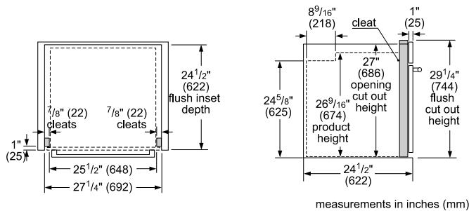
Flush Install Top View
