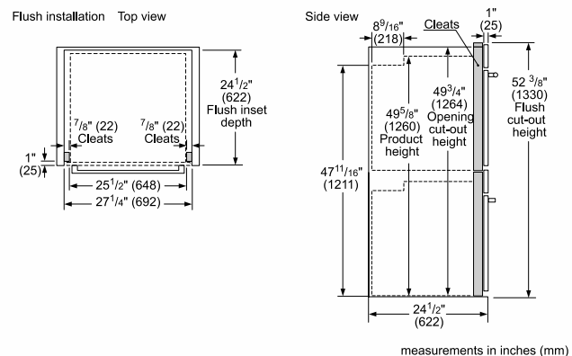
Flush installation Top view
