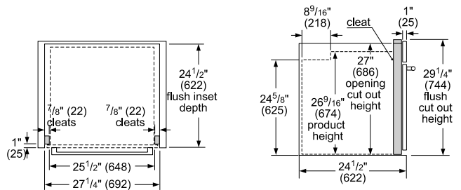
Flush Install Top View
