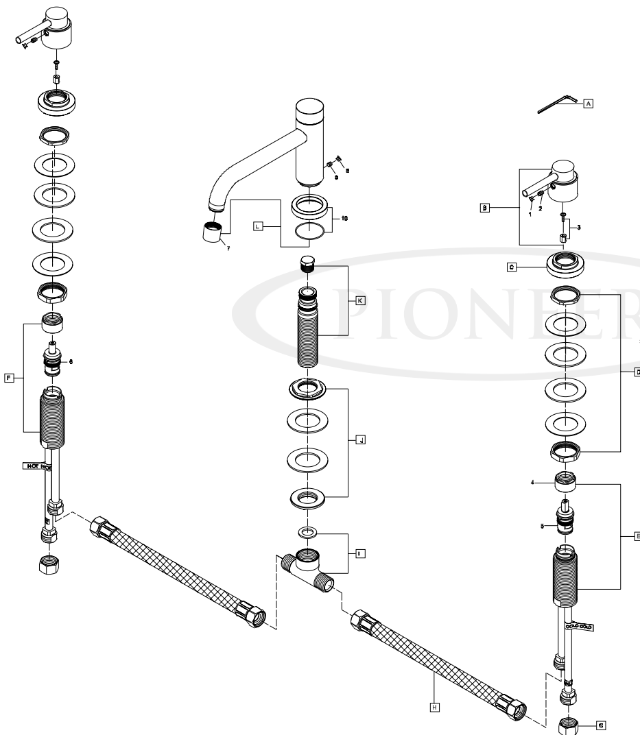
Product Diagram
