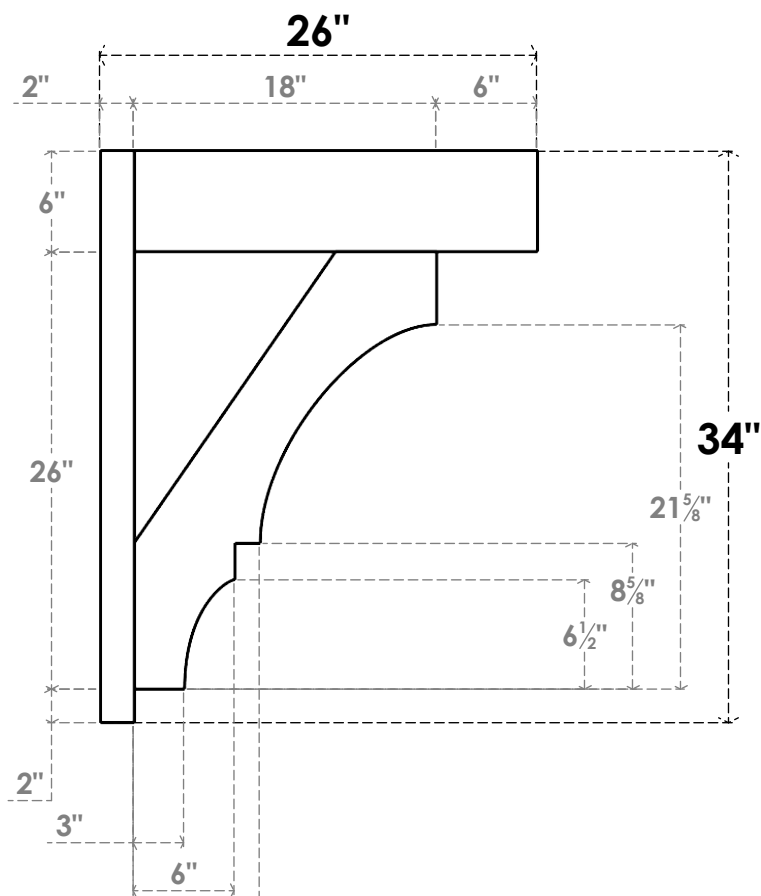
SIDE PROFILE
