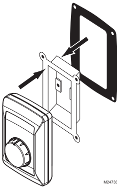
Fig. 14. Slide the foam gasket onto the base.
