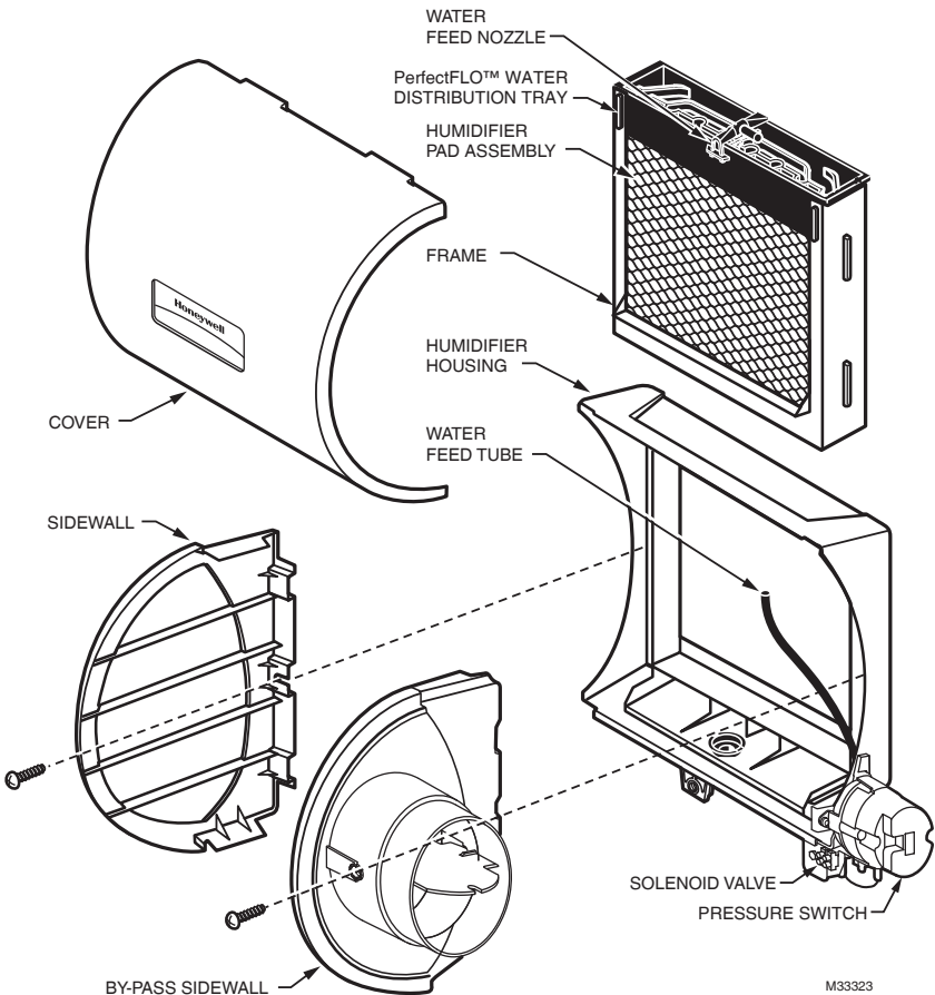
Fig. 4. Disassembling humidifier.
