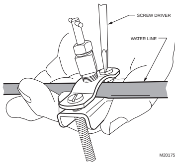
Fig. 8. Installing the saddle valve.
