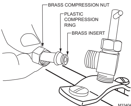
Fig. 9. Installing feed tubing.
