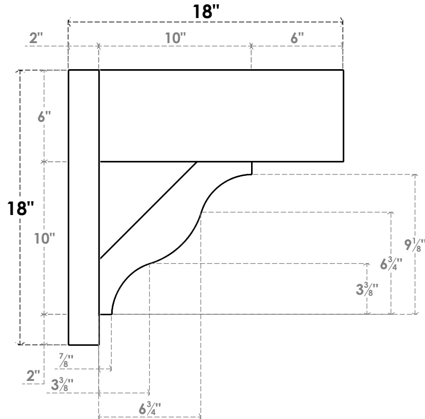
SIDE PROFILE
