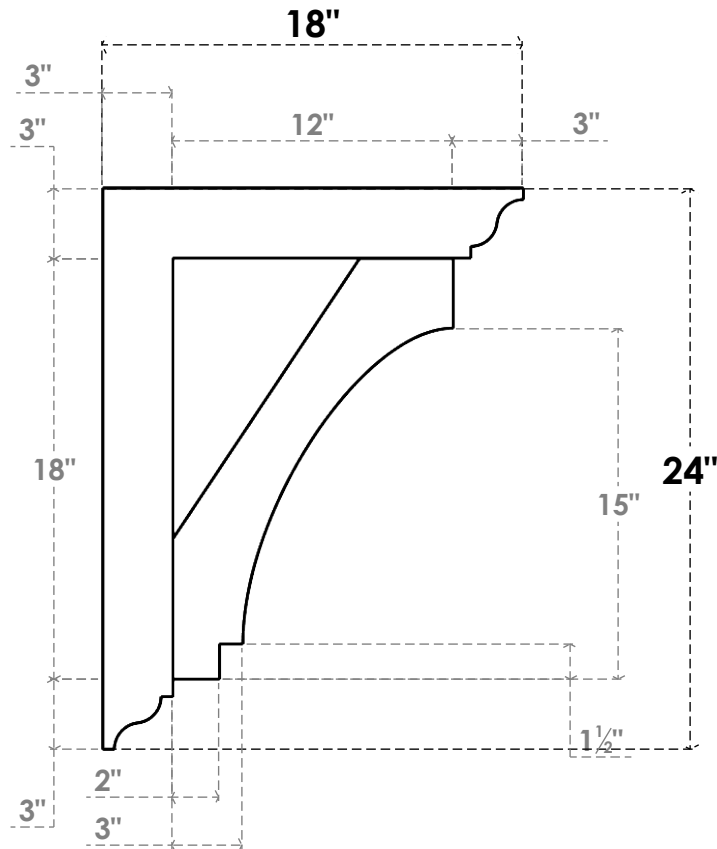
SIDE PROFILE
