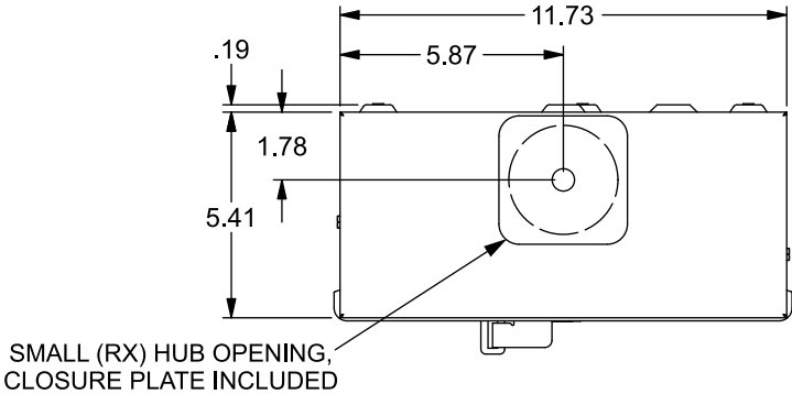
VIEW SHOWN WITH LOWER COVER REMOVED
