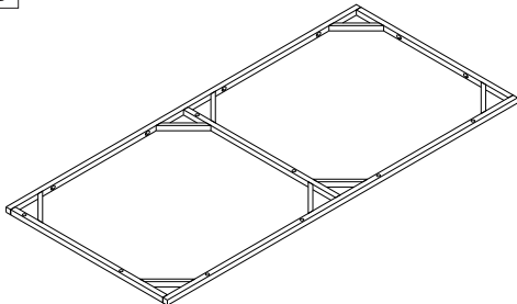
Inner frame (2 pcs)
