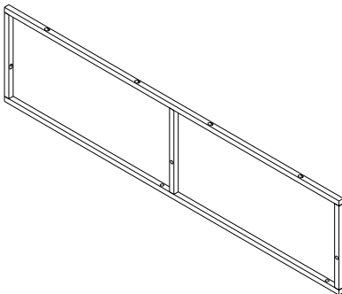
Front frame (1 pc)
