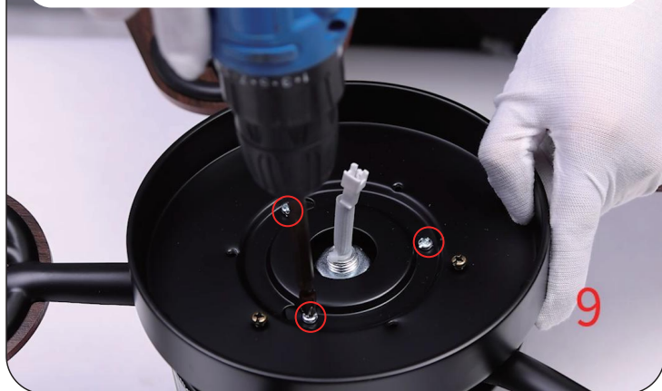
9. Insert the third light kit screw, and then tighten all three light kit screws
