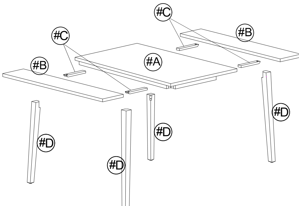
Support bar
