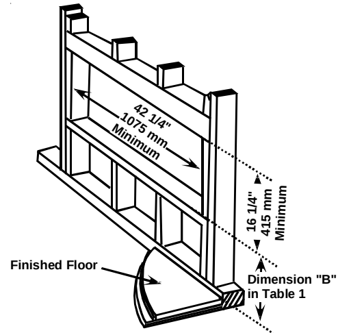
Figure 2 - Minimum Wall Opening Dimensions
