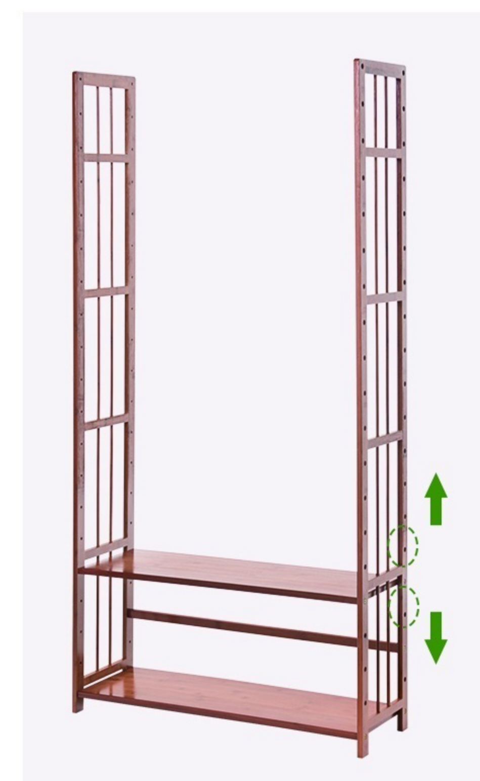
④ Installation of laminates and screws as shown ( The hole is reserved, and the laminate can be adjusted up and down. )
