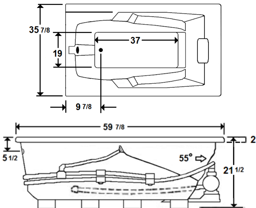
Standard Pump & Heater Location
