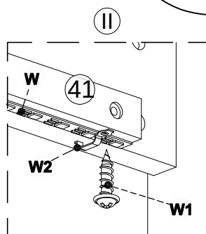
LED LIGHT CONNECTION WIRE / LUMIÈRE LED FIL DE CONNEXION
