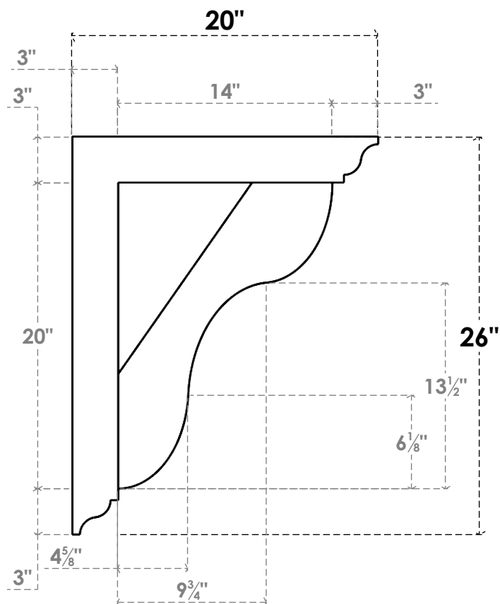
SIDE PROFILE
