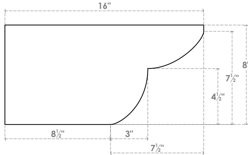
SIDE PROFILE
