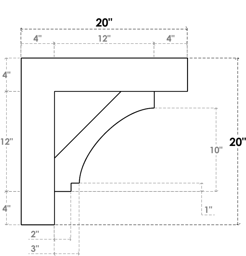
SIDE PROFILE
