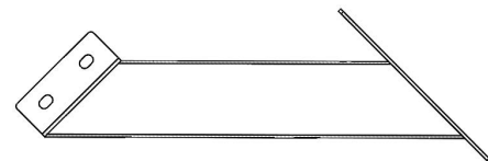
F4 | SHORT ANGLE BRACE - A4M01276 (2) 1\frac{1}{8} \times 4 \times 14 (30x101x355)
