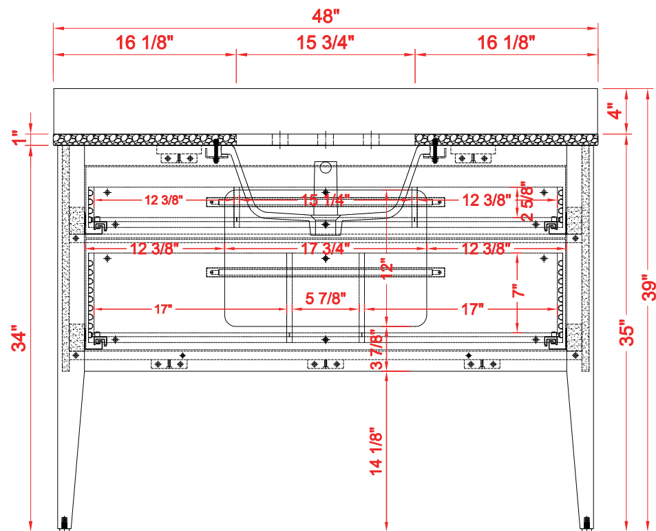
FRONT VIEW
