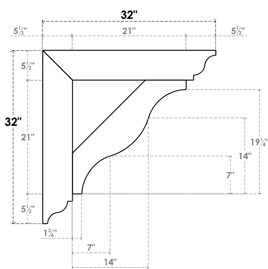
SIDE PROFILE
