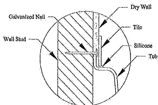
Integral Flange
