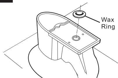
Install Wax Ring (not provided).
