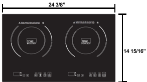
Cooktop Dimensions
