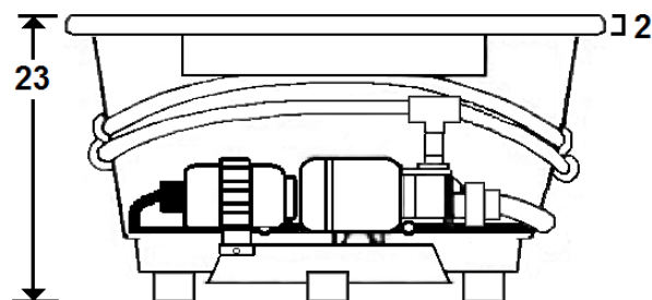
Standard (S) Pump, Blower, & Heater Location
