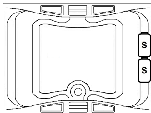
Standard (S) Pump, Blower, & Heater Location
