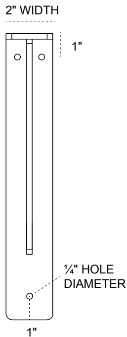
FRONT PROFILE
