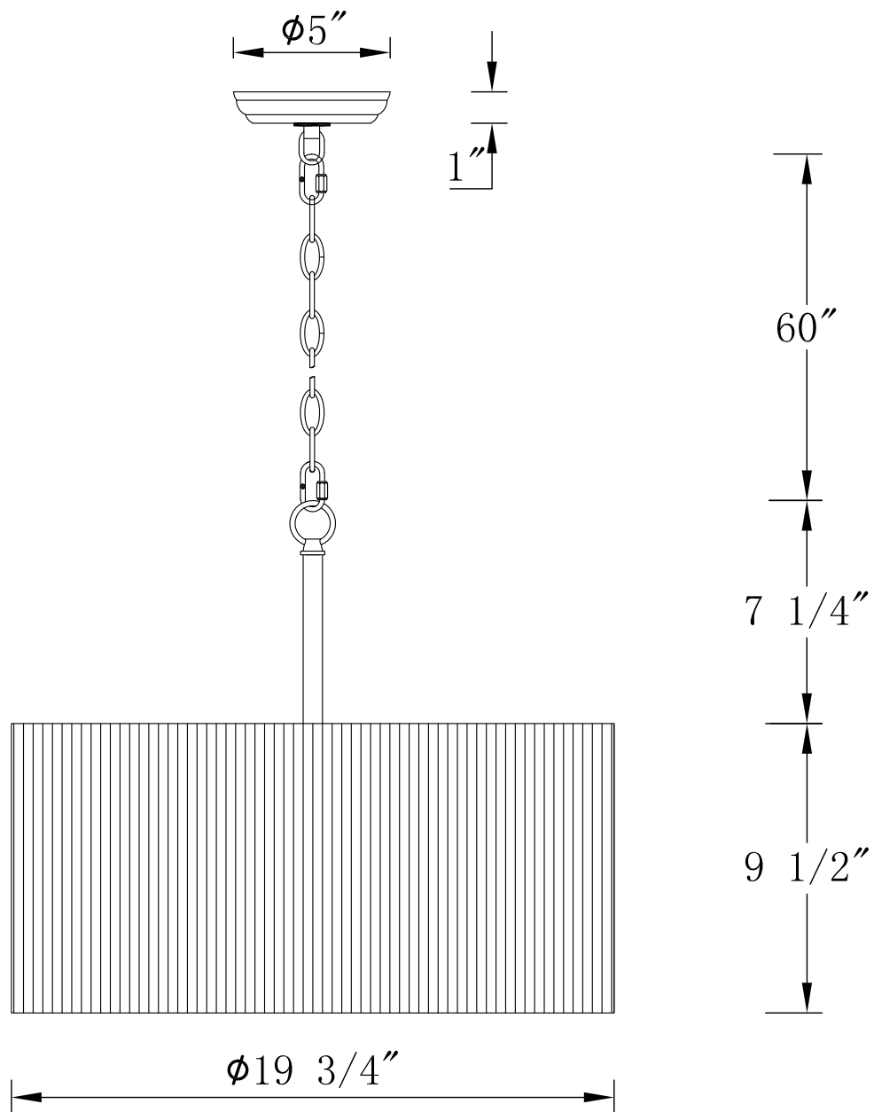
FRONT VIEW
