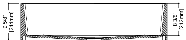
VISTA FRONTAL
