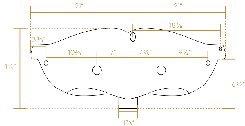
BACK
