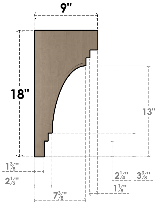
SIDE PROFILE
