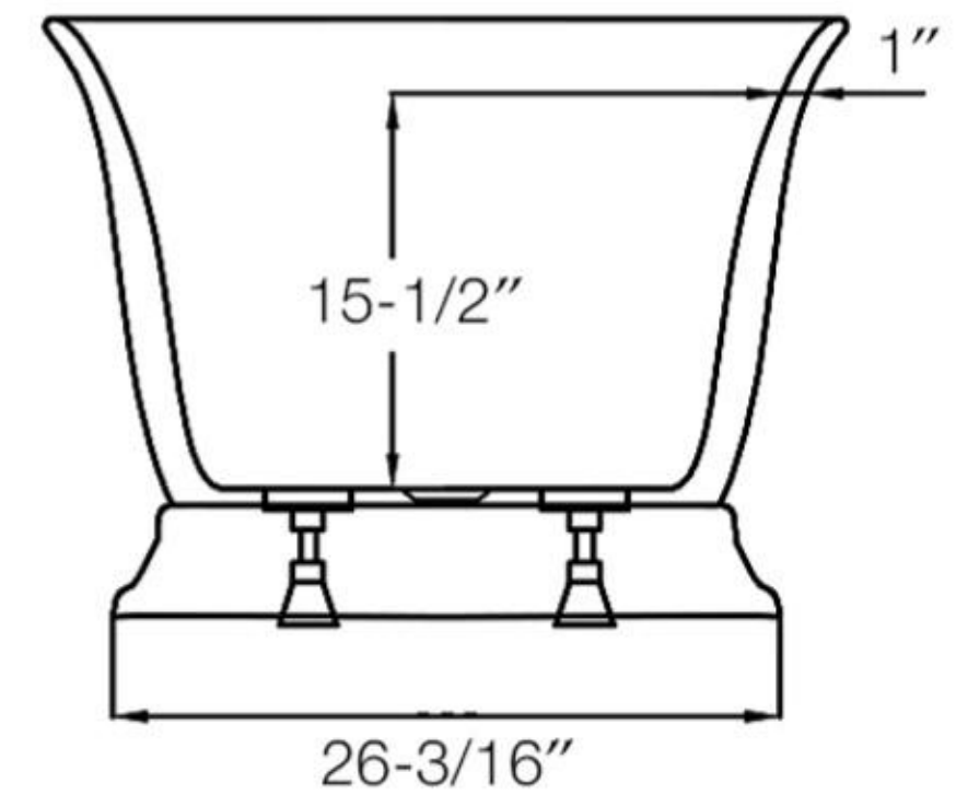
Side View
