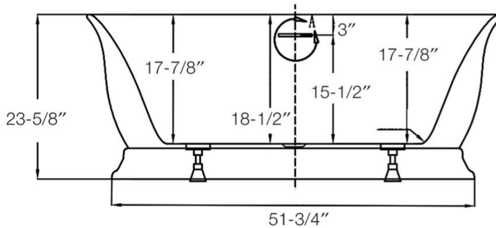
Front View
