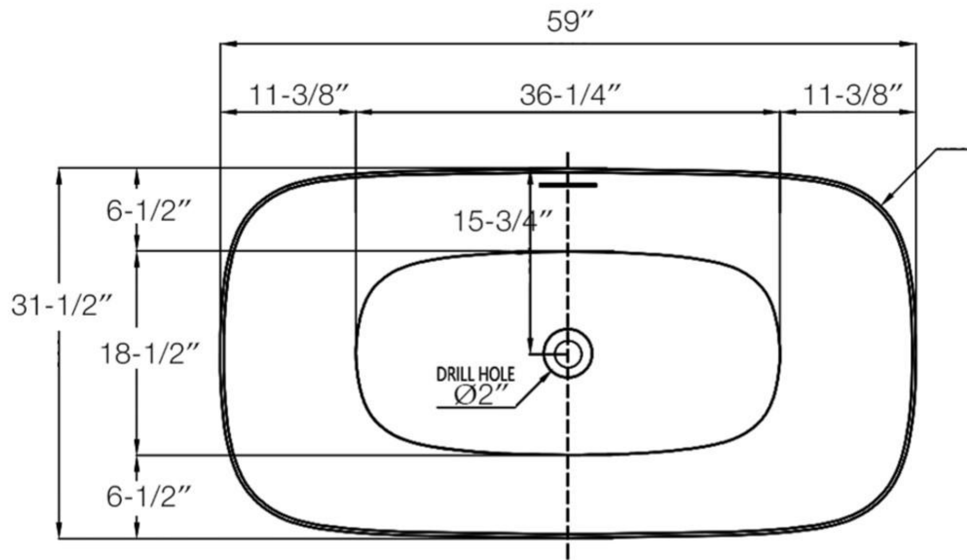
Top View
