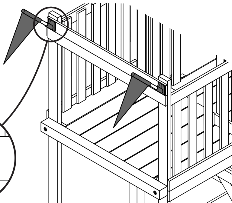
FRONT SIDE
