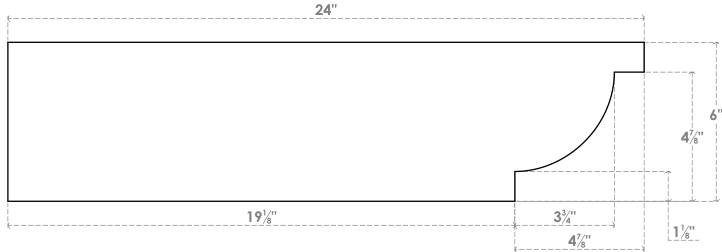
SIDE PROFILE
