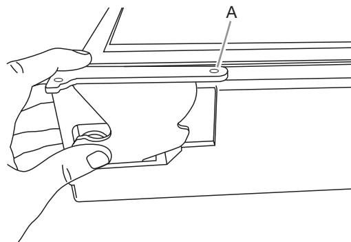
A. Hinge base parallel to the bottom edge of the door
