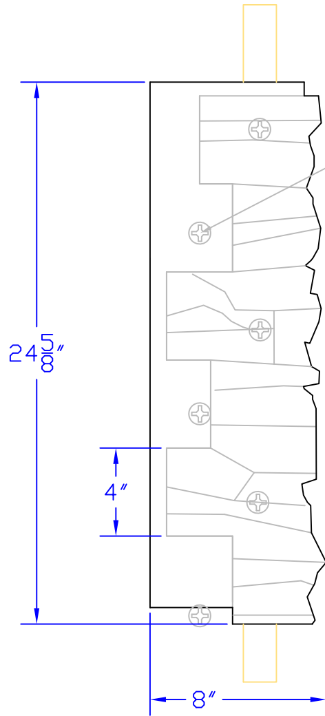
Left View
