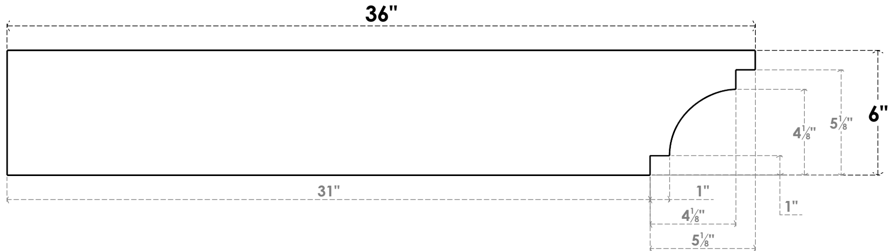
SIDE PROFILE
