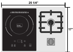
Cooktop Dimensions
