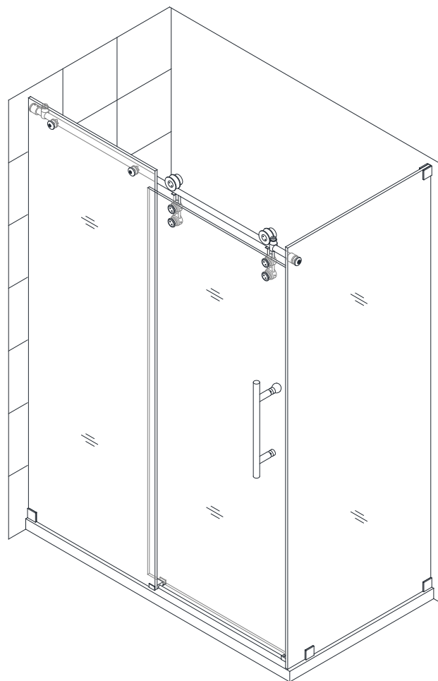
Right-hand return panel installation
