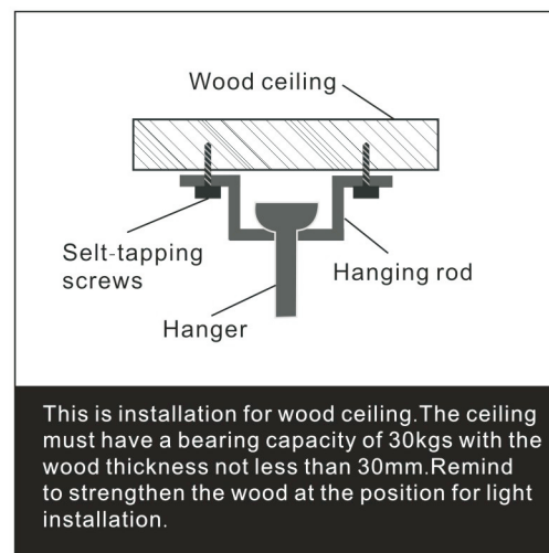
Diagram 4: Installation with wood decorative ceiling
