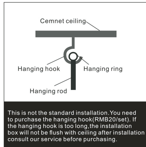
Diagram 2: Installation with hook
