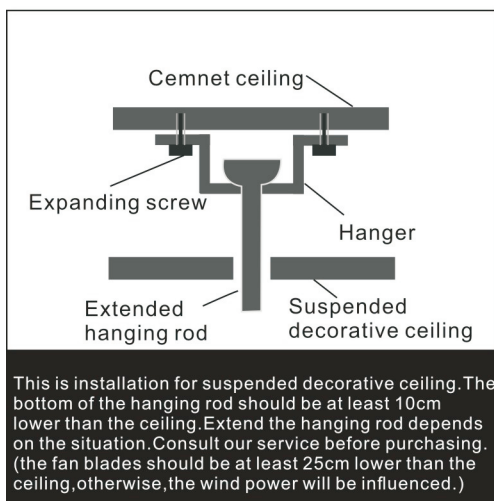
Diagram 3: Installation with suspended decorative ceiling
